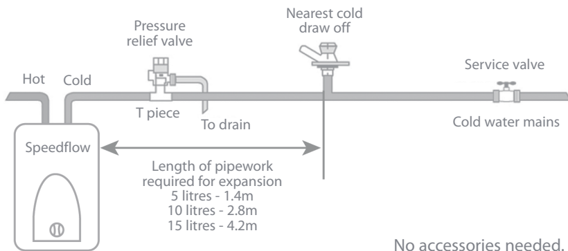
DIAGRAM A - Pressure below 4.2 bar
